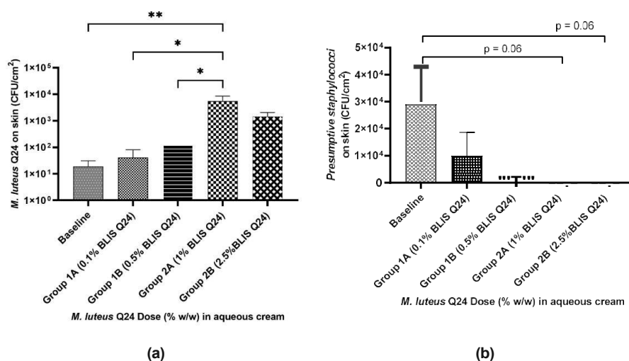
Figure 6. Influence of M. luteus Q24 dosage level on the subsequent colonisation levels of (a) M. luteus Q24 and (b) presumptive staphylococci , detected 24h post last dose following one week of pre-sleep application on the face of adult participants ( n = 9 ). Low dose group ( n = 5 ) High dose group ( n = 4 ). Data points are means \pm SD. Only groups showing a significant difference are indicated on the graph with one* indicates p < 0.05 and ** indicates p < 0.01 .
